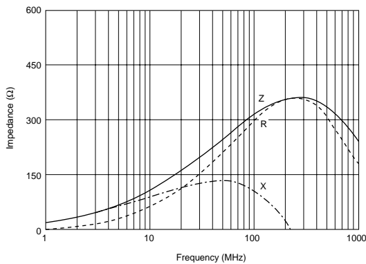
BLM18PG331SN1
